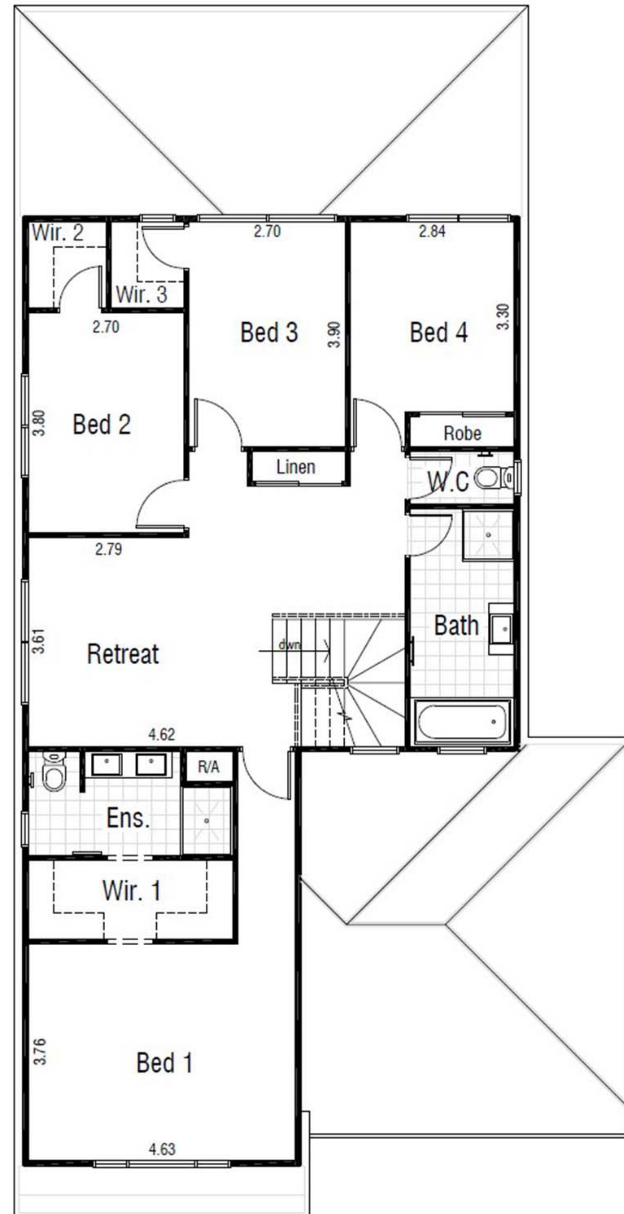
FIRST FLOOR
