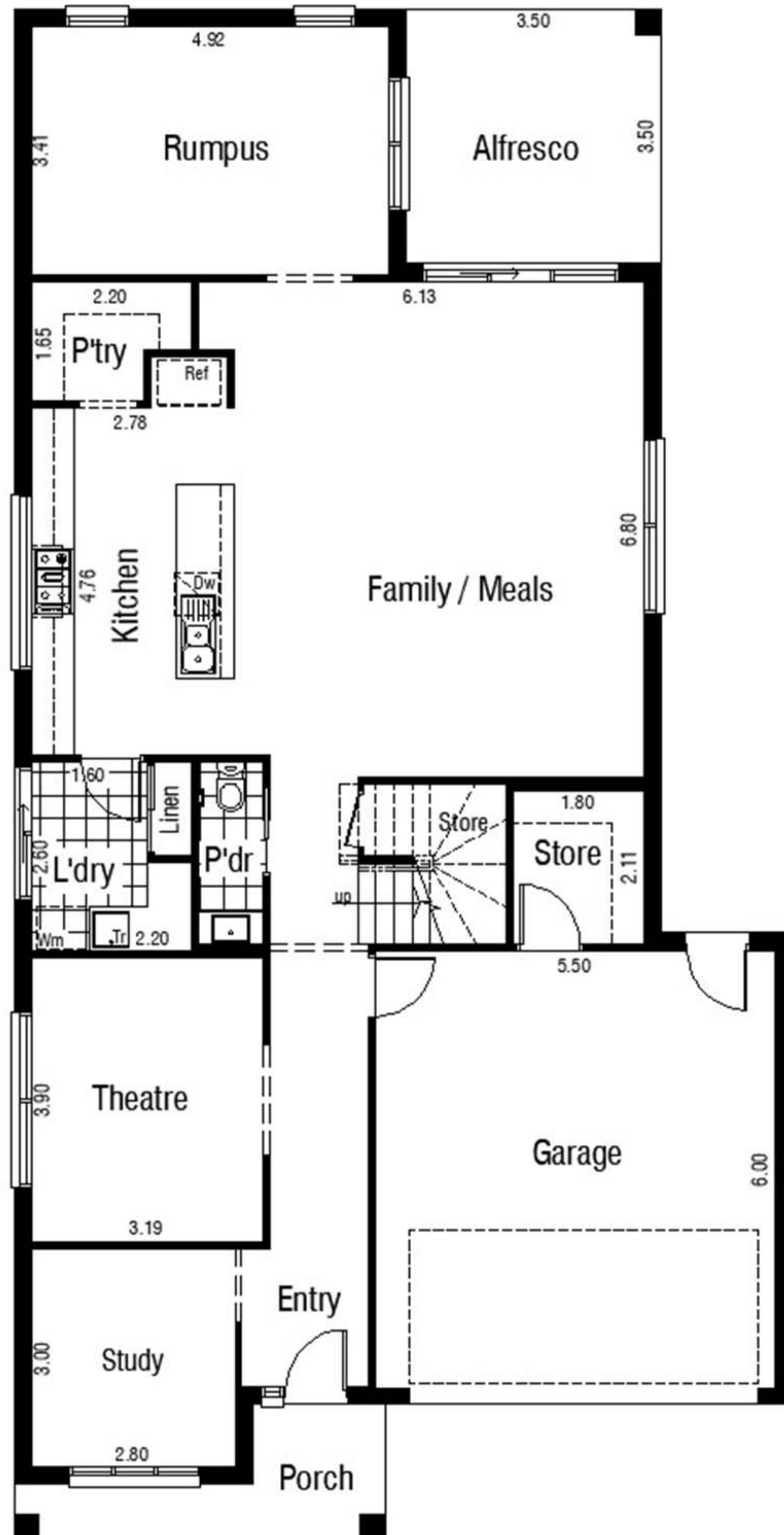
GROUND FLOOR
