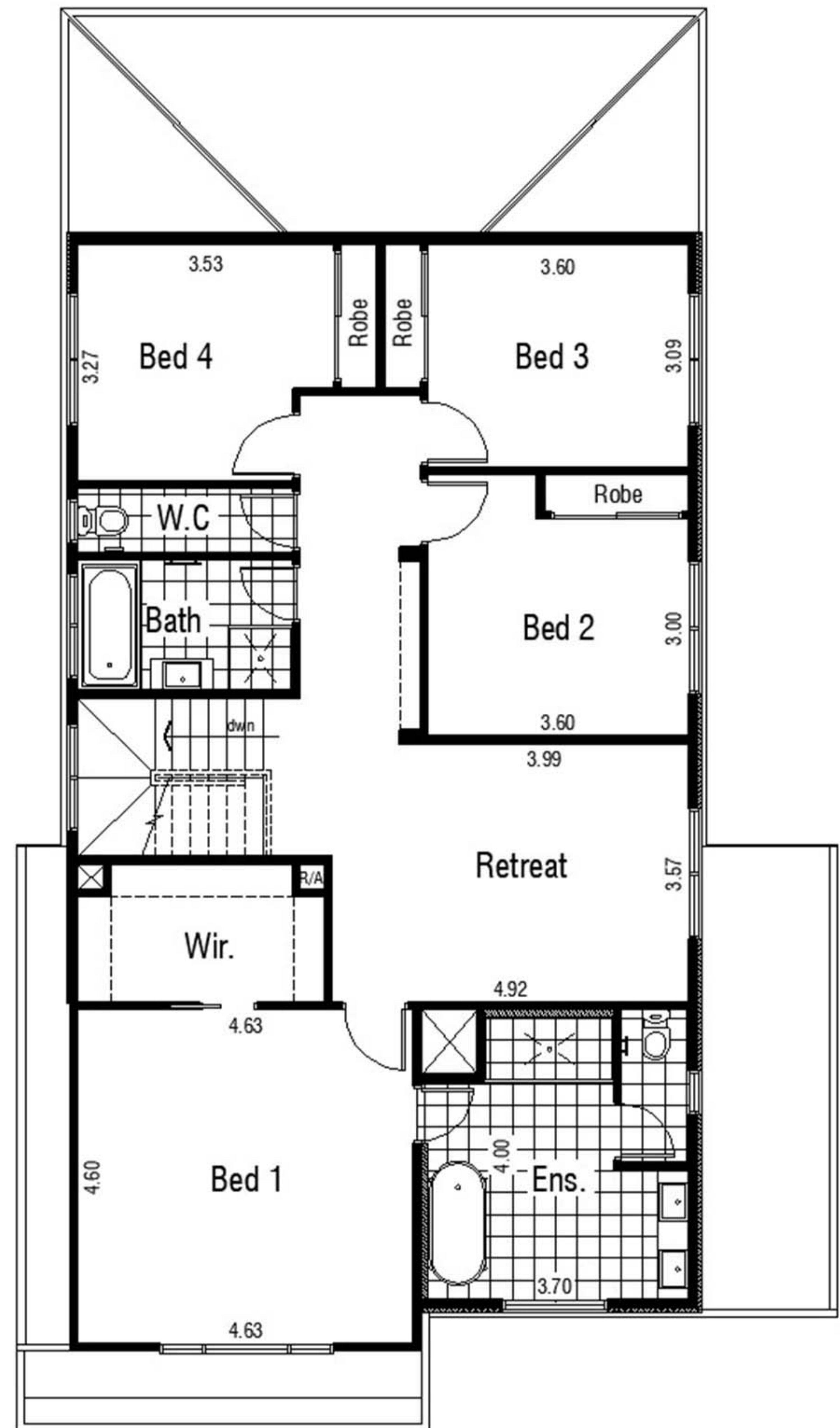
FIRST FLOOR
