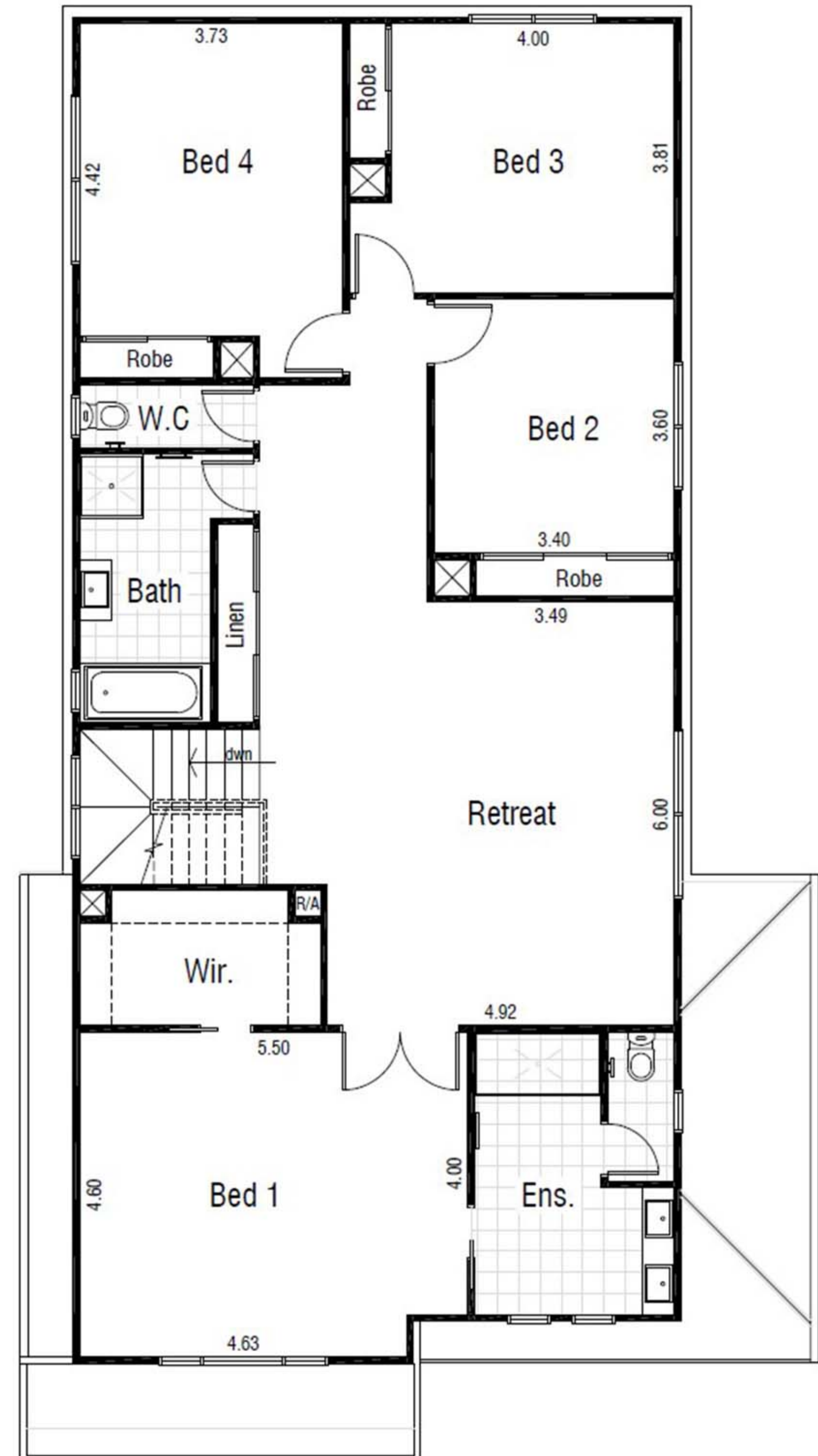
FIRST FLOOR
