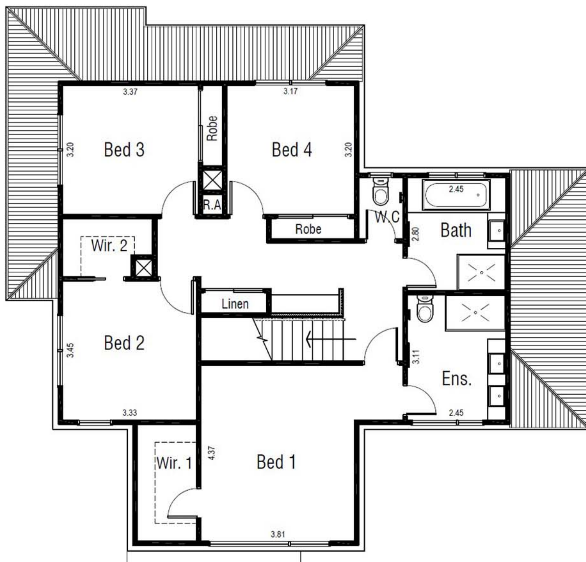
FIRST FLOOR
